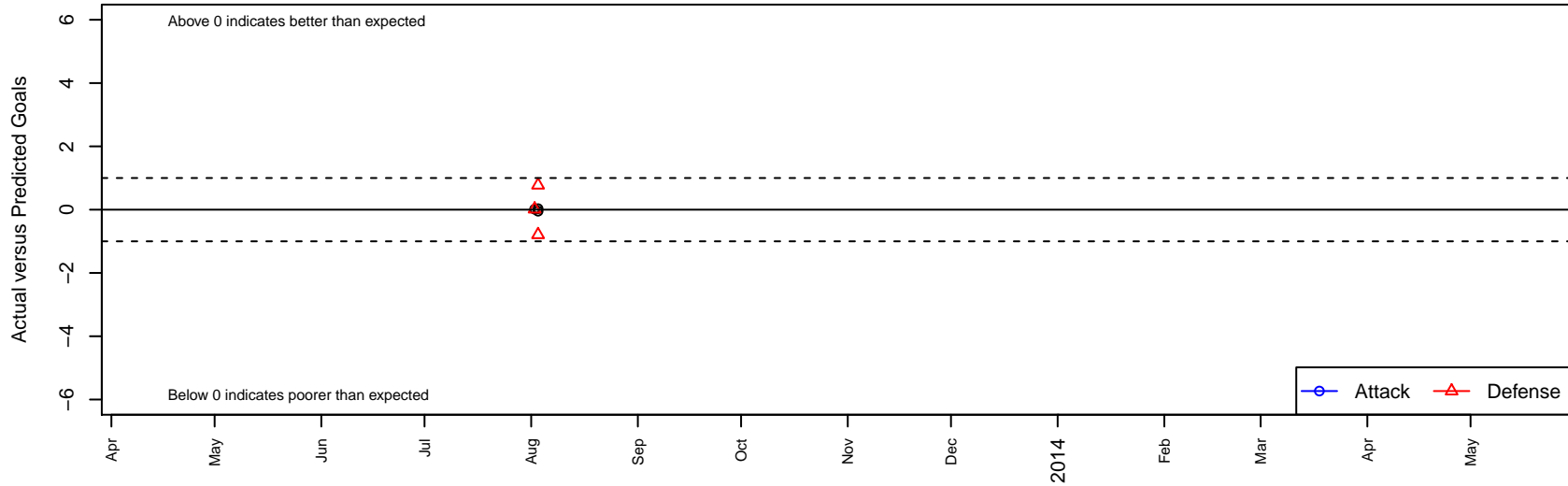
Aztec Sungods B94 Dots are actual minus expected GF (blue circles) and GA (red triangles). Blue line is smoothed change in attack strength. Red is smoothed change in defense strength.
